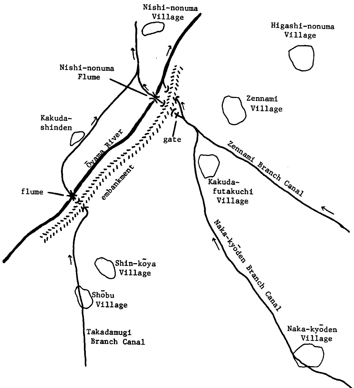
Map 8; Sketch map of the Kakuda-futakuchi area
